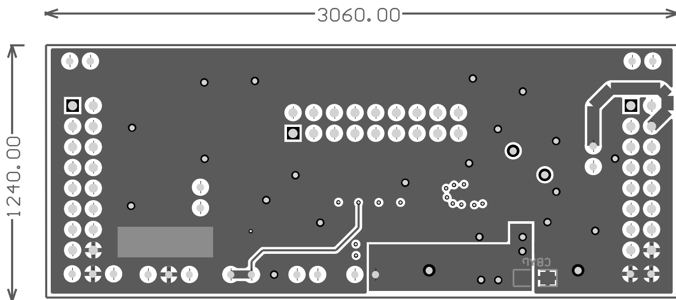
Figure 5. Bottom Layer
