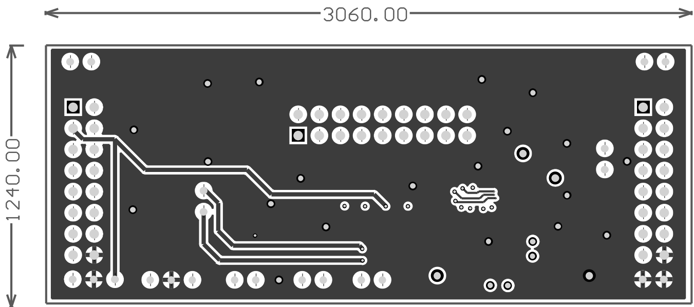
Figure 3. Mid Layer 1
