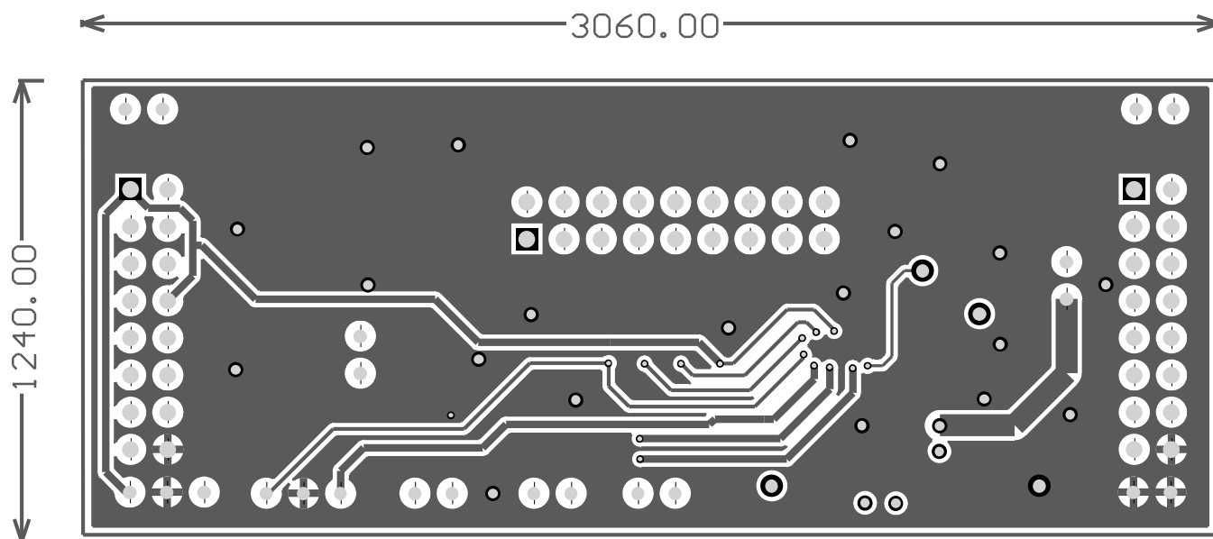
Figure 4. Mid Layer 2
