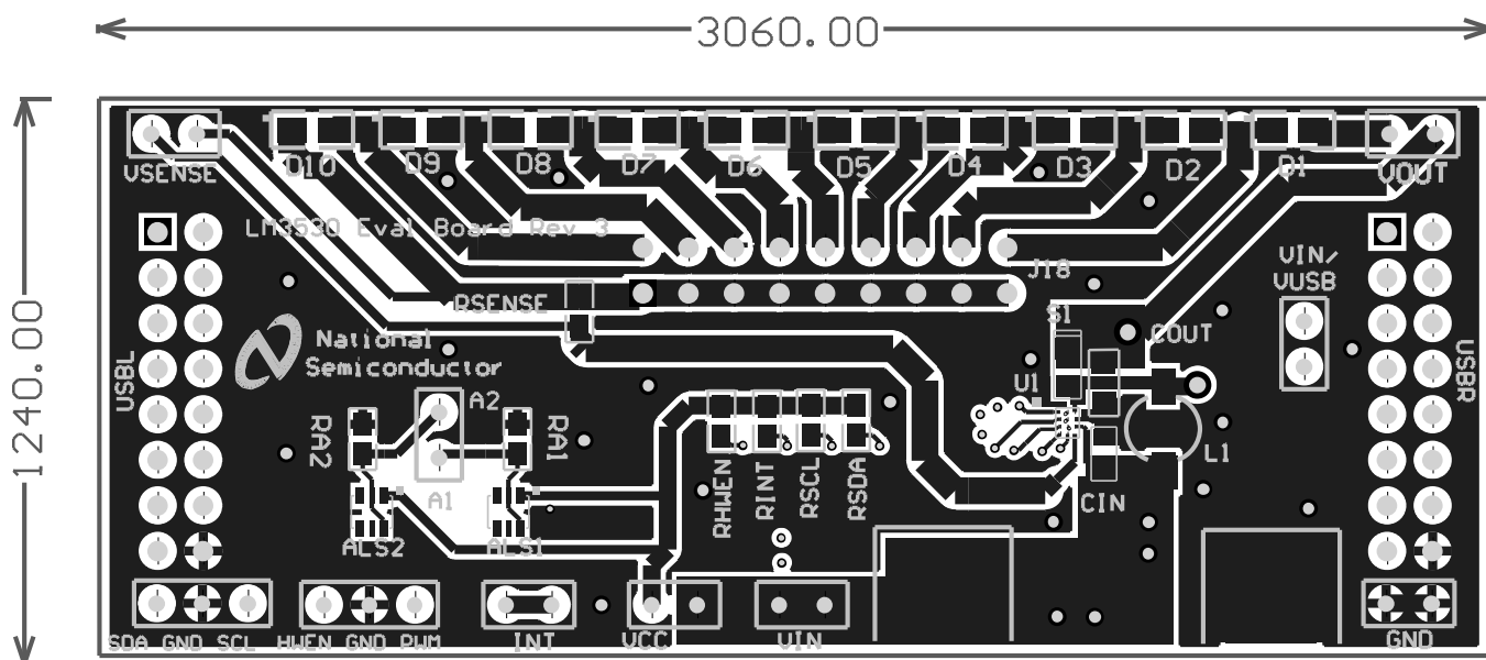
Figure 2. Top Layer
