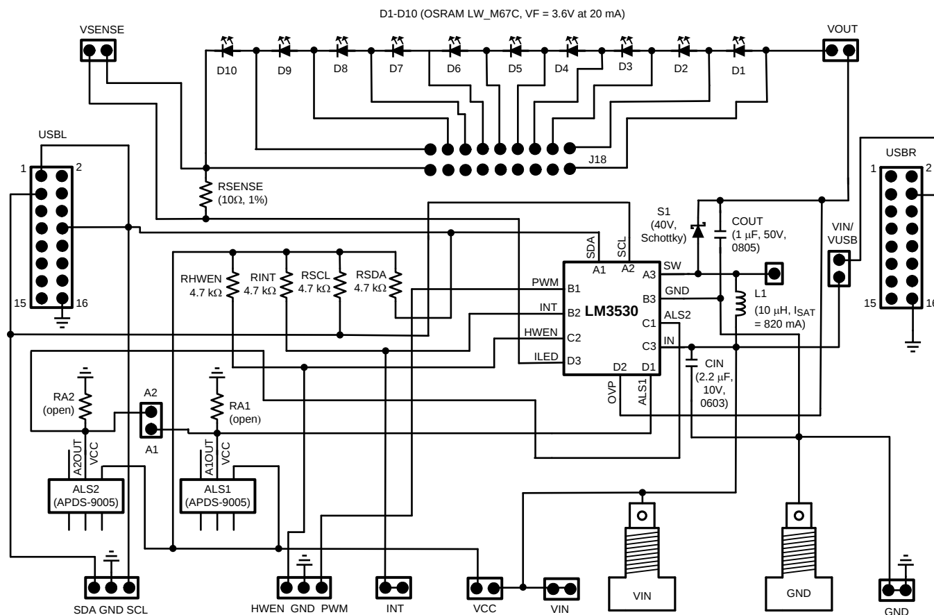
Figure 1. LM3530 Evaluation Board Schematic
