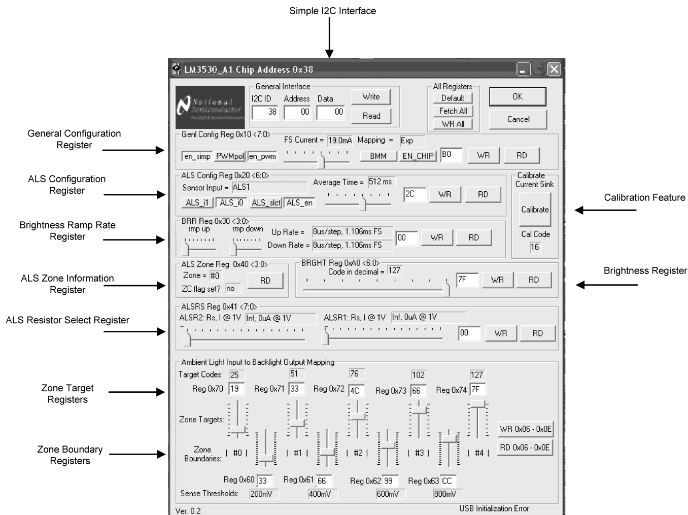
Figure 6. LM3530.exe Program
